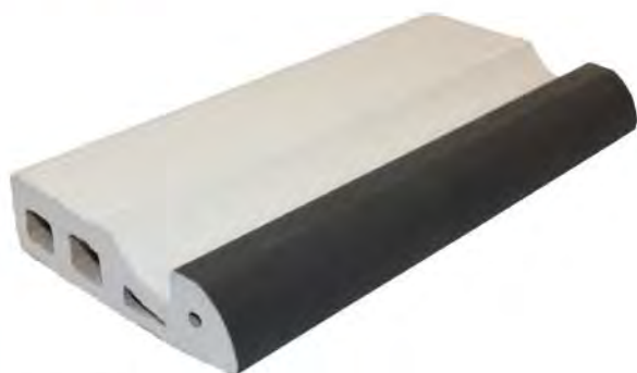
Solid Finnish Edge 12x25cm - 35mm
