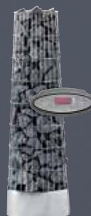
KIVI Output: 6,9–9,0 kW Sauna room: 6–14 m 3
